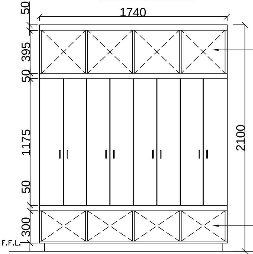
INSIDE ELEVATION
