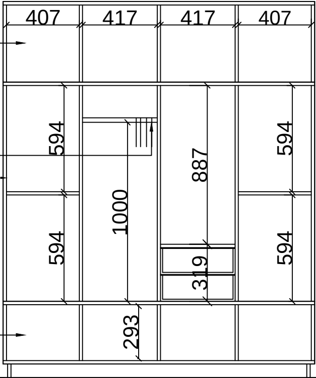
FRONT ELEVATION
